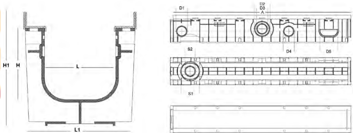
SABDRAIN 707
